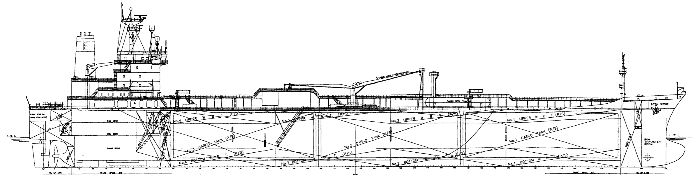
BRIDGE FRONT VIEW & TANK SECTION
